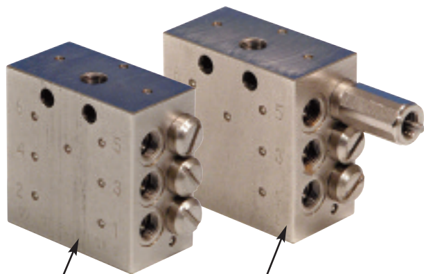
Divider valves with visual indicator pin
